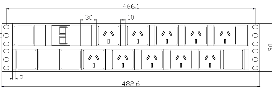
RPR-10HMCB: Front View
