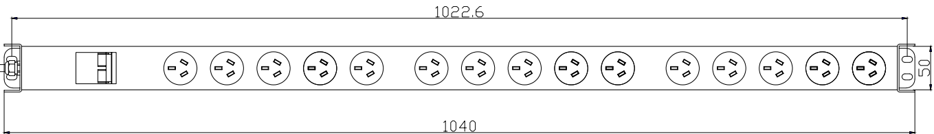
RPR-15VMCB: Front View
