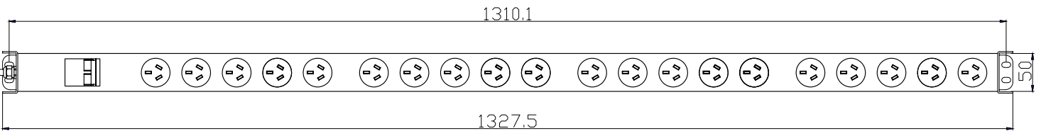
RPR-20VMCB: Front View
