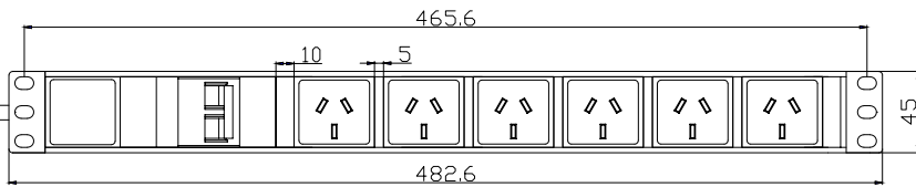
RPR-6HMCB: Front View
