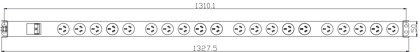
RPR-20V15MCB: Front View
