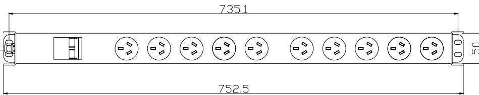
RPR-10V15MCB: Front View
