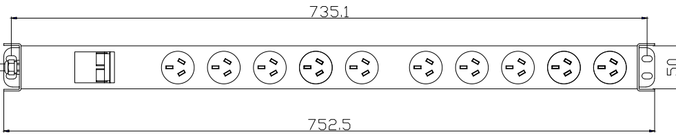
RPR-10VMCB: Front View
