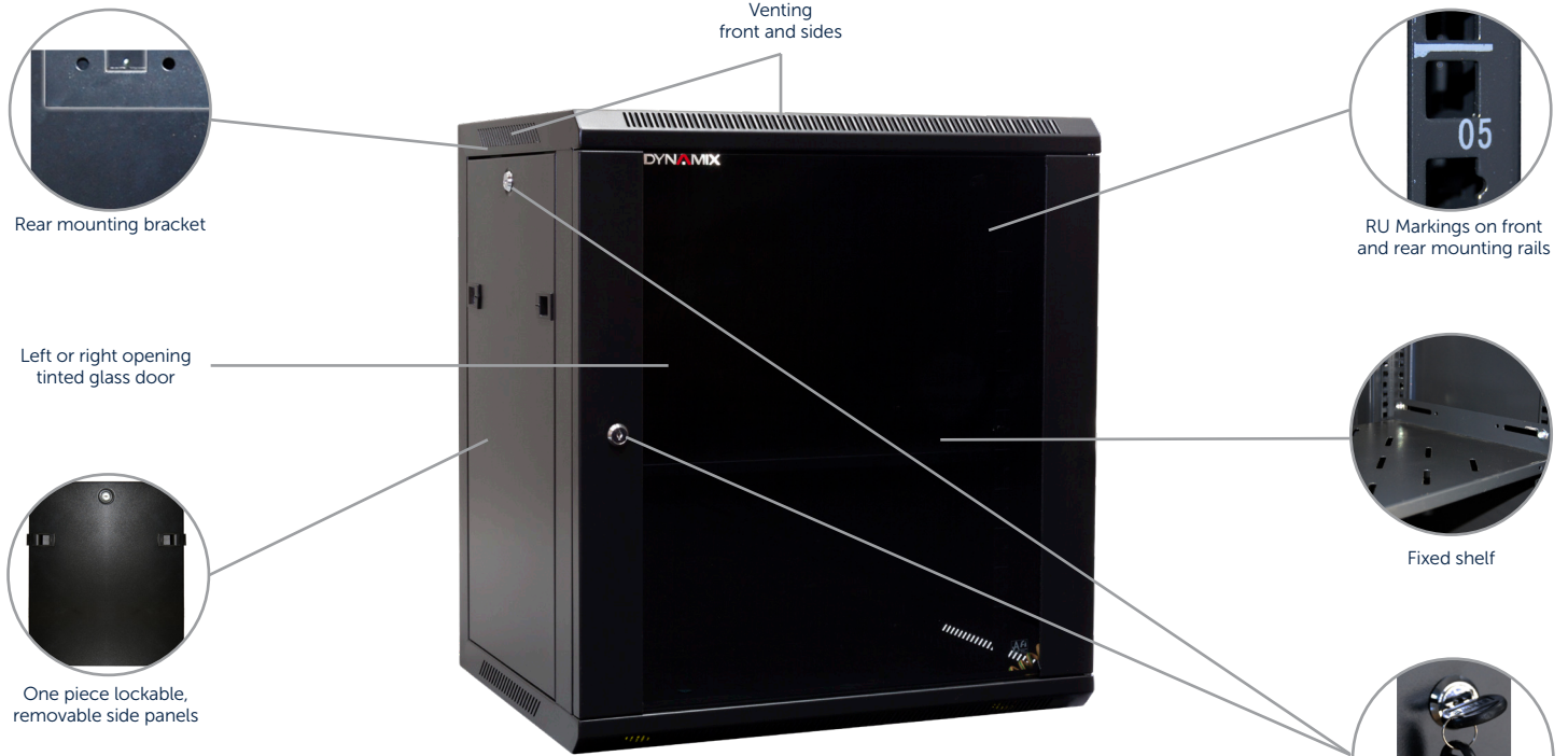
CABINET FRONT
